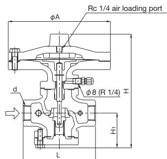
Screwed type
